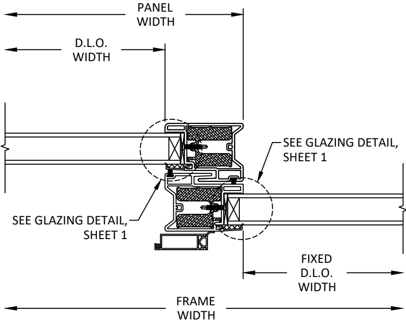
B 6 HORIZONTAL SECTION INTERLOCK
