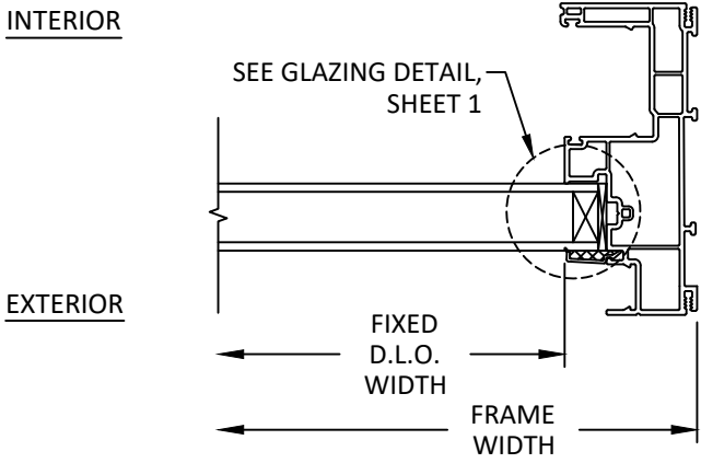
C 6 HORIZONTAL SECTION FIXED JAMB REPLACEMENT FRAME
