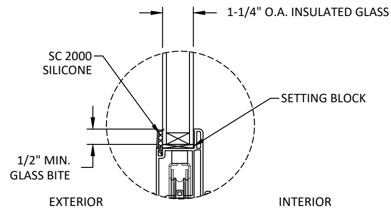
GLAZING DETAIL 1
