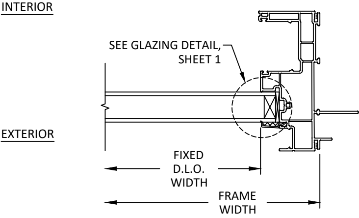
E 6 HORIZONTAL SECTION FIXED JAMB NEW CONSTRUCTION FRAME
