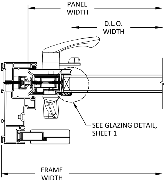
A 6 HORIZONTAL SECTION LOCK JAMB REPLACEMENT FRAME
