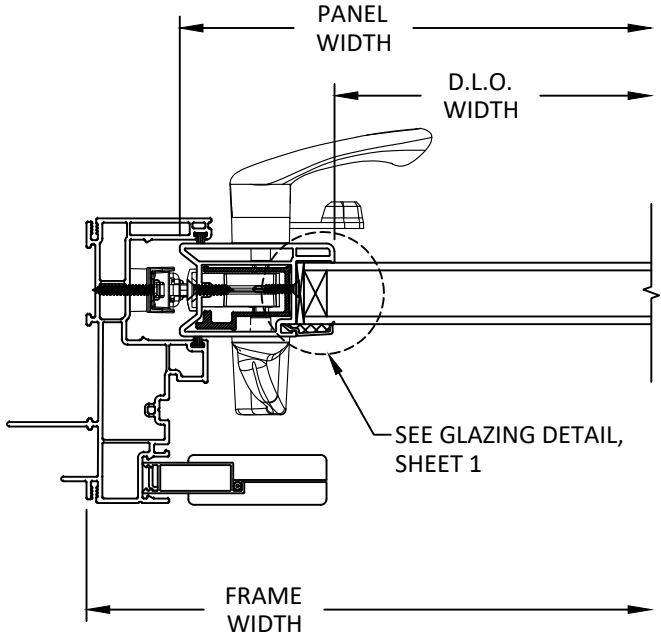
D 6 HORIZONTAL SECTION LOCK JAMB NEW CONSTRUCTION FRAME
